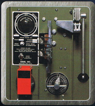
RWA Butt Welder
