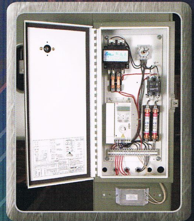
Electronic Panel with Frequency Drive
